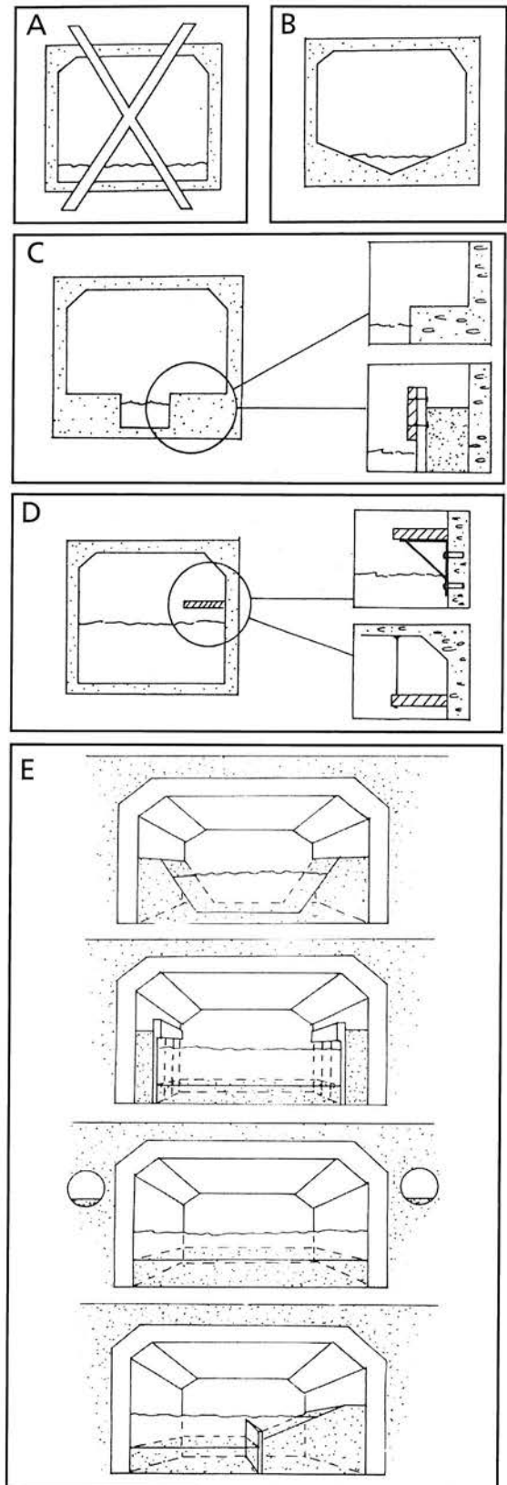
Figure 7.59 - Small terrestrial animals can use culverts, if dry walkways are provided. A: not suited for terrestrial animals, because water covers the whole bottom part of the culvert. B and C: prefabricated concrete walkways above the water level. D: a wooden board above the water level, fixed to the side wall. E: design perspectives.
