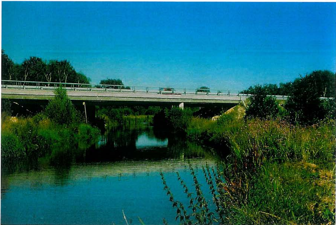
Figure 7.43 - A river crossing in France which preserves the natural river bed and has dry banks for movements by terrestrial animals. (Photo by J. Carsignol)
