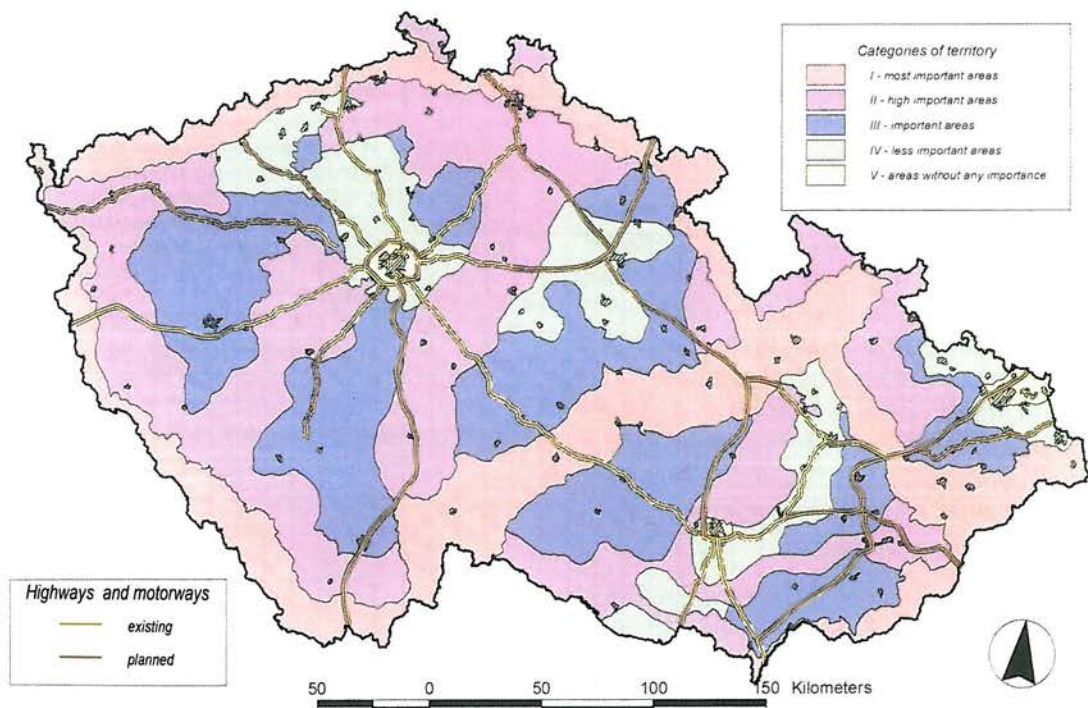
Figure 7.8 - Categorisation of the territory of the Czech Republic according to importance for mammals.
