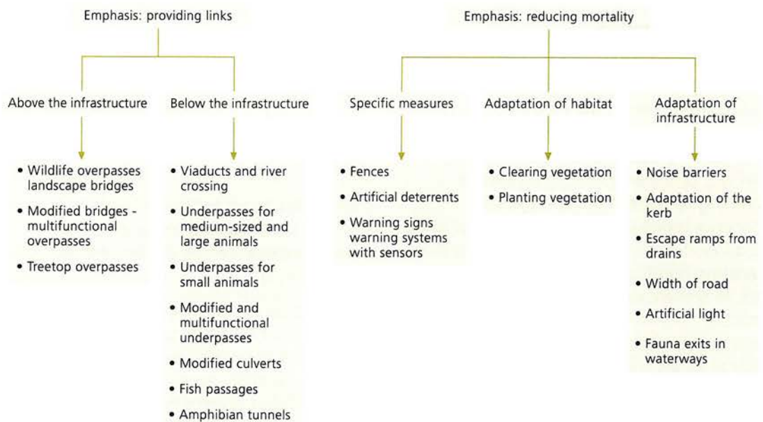
Figure 7.1 - Types of measures to mitigate habitat fragmentation.
